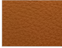
pelle cristal: 65
