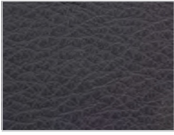
pelle cristal: 13
