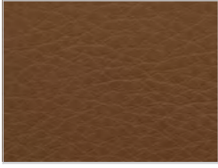
pelle cristal: 49
