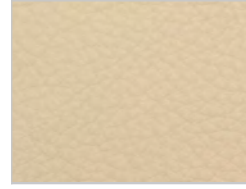
pelle cristal: 70
