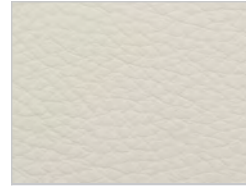
pelle cristal: 18
